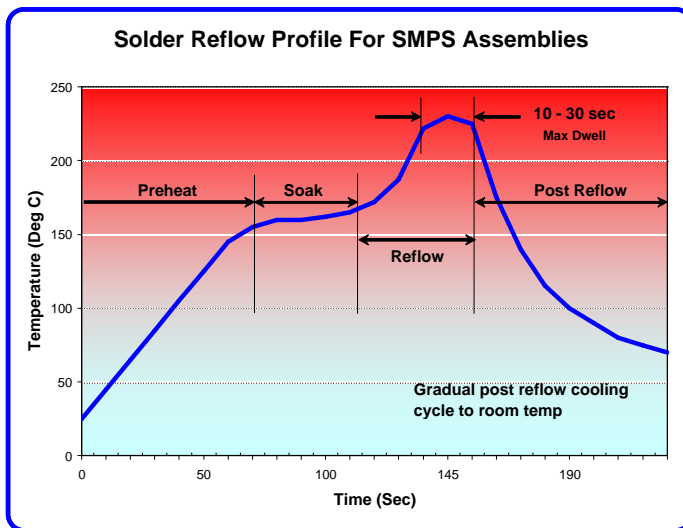
Figure 1 – Typical Solder Reflow Profile for SMPS Capacitor Assemblies
